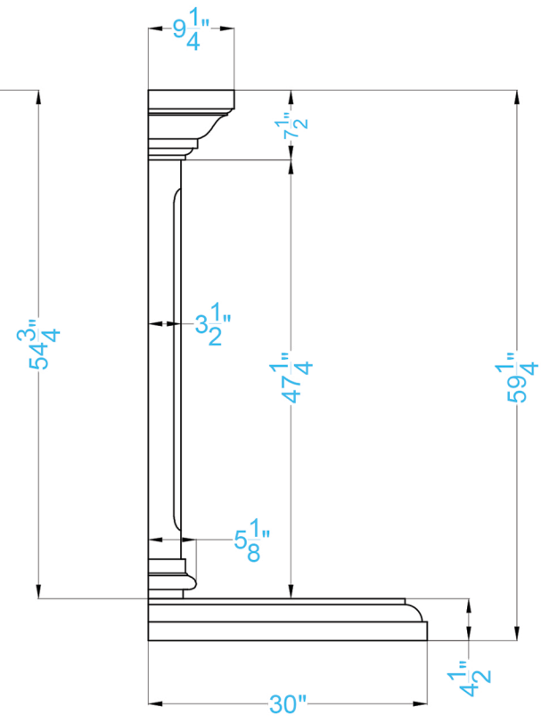
SIDE VIEW
