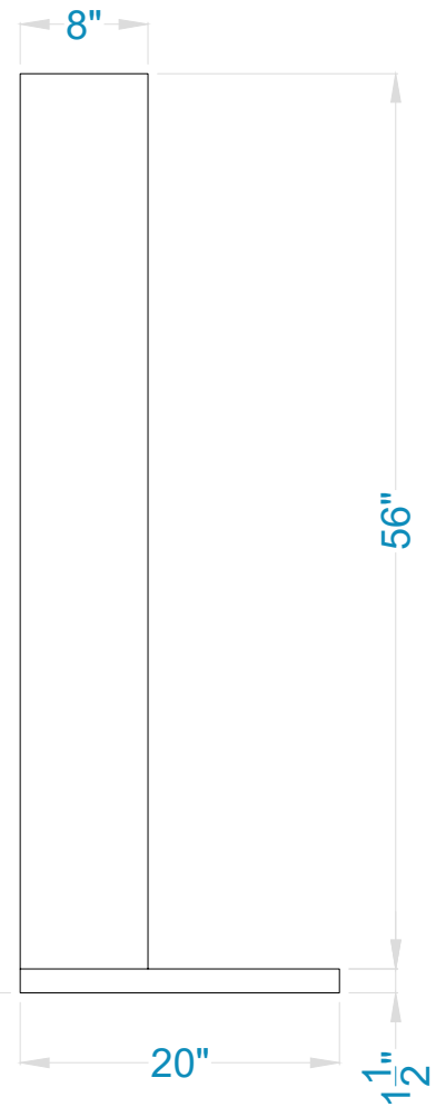
SIDE VIEW
