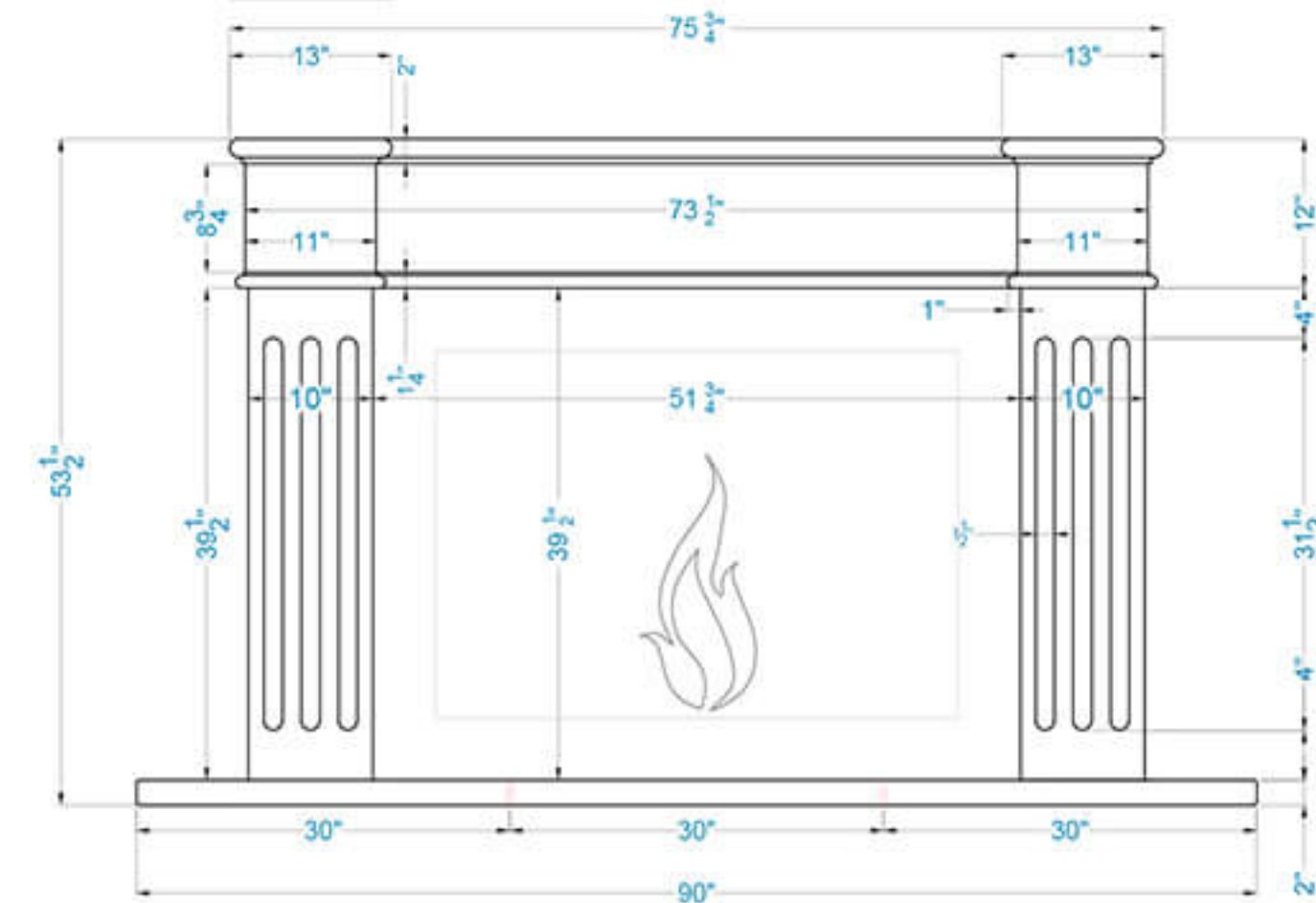
FRONT VIEW
