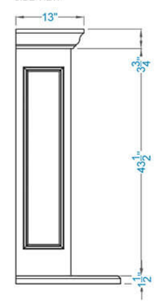
SIDE VIEW
