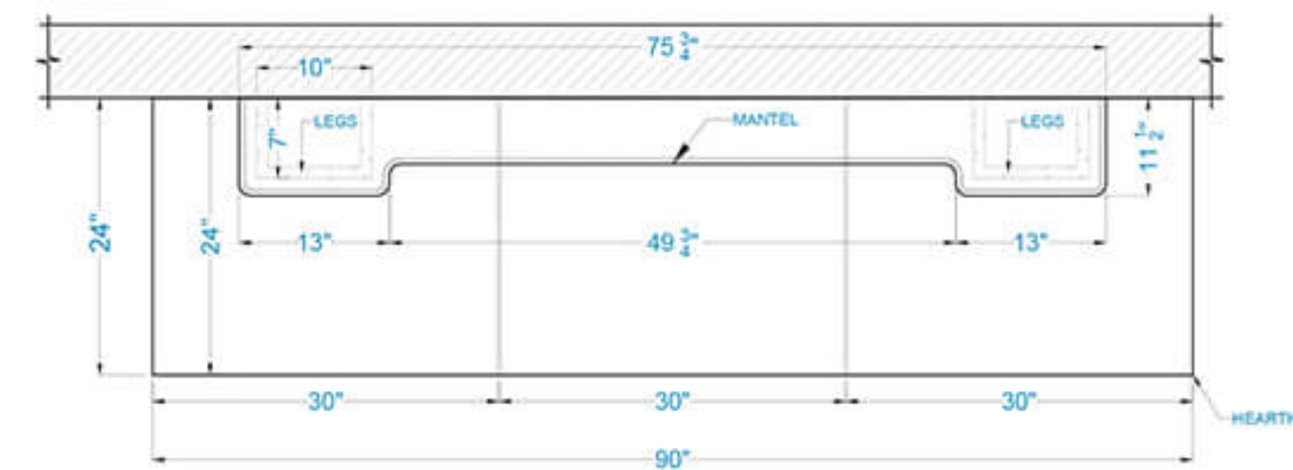
FRONT VIEW
