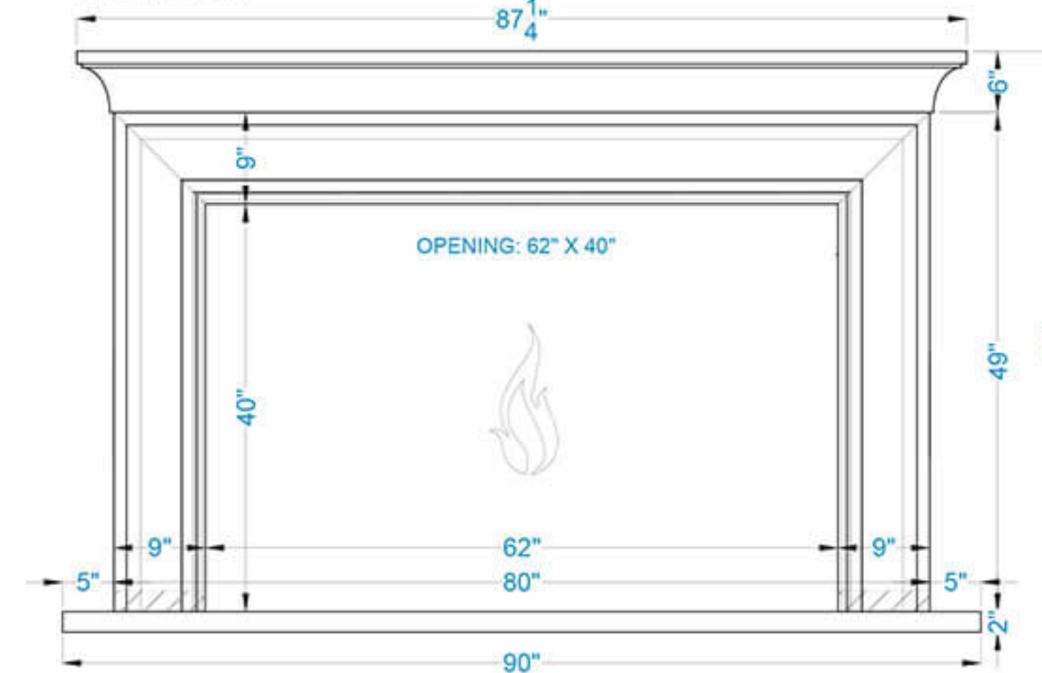
FRONT VIEW
